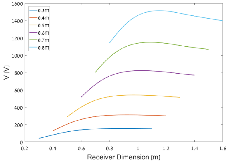
Figure 15: Voltage across receiver as a function of the change in DD coil dimensions. Different curves represent different transmitter coil dimensions from 0.3 to 0.8 m.
