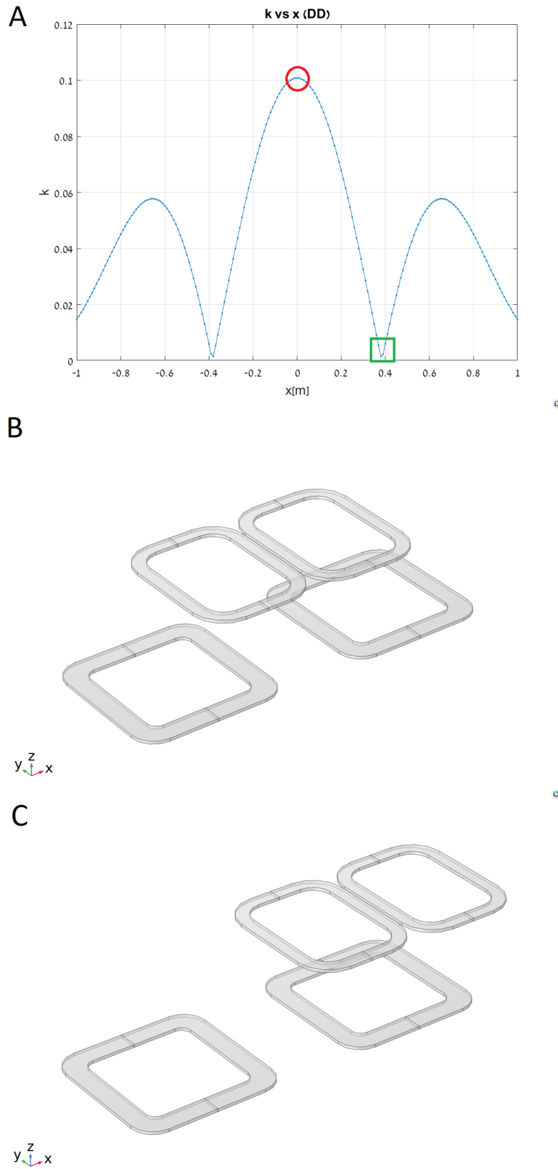
Figure 9: 'DD' configuration shift effects. A: Changes to k as a function of misalignments along the travel path. The red circle represents the configuration shown in B, and the green rectangle represents the configuration shown in C. In both cases, the receivers
