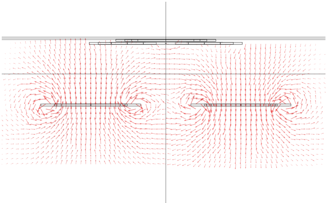
Figure 7: An example of the flux lines of a bipolar configuration, simulated by us. Each transmitter pair is applied a clockwise and counterclockwise current in a 'figure of eight' manner, resulting in an alternating positive-negative field. This method is preferred since it has less flux gaps in-between the coils.
