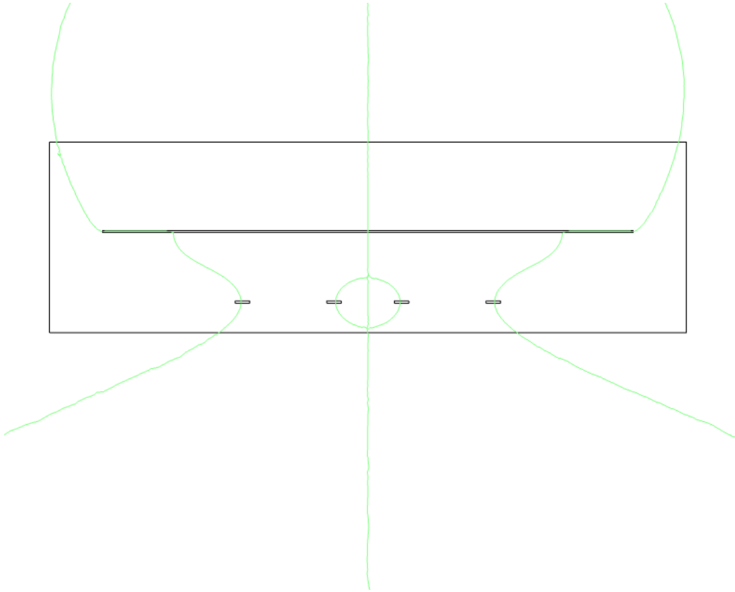
Figure 20: A side view of the system. The green line represents every point where B_z = 0 , meaning the flux direction flips in every region.
