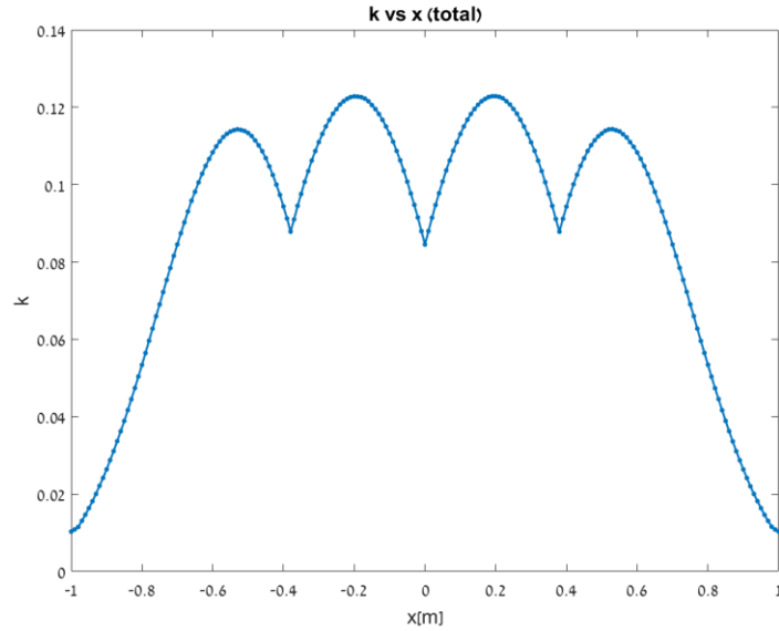
Figure 33: Changes to k at different x -axis misalignments. Consistently good k values are obtained throughout the entire movement.
