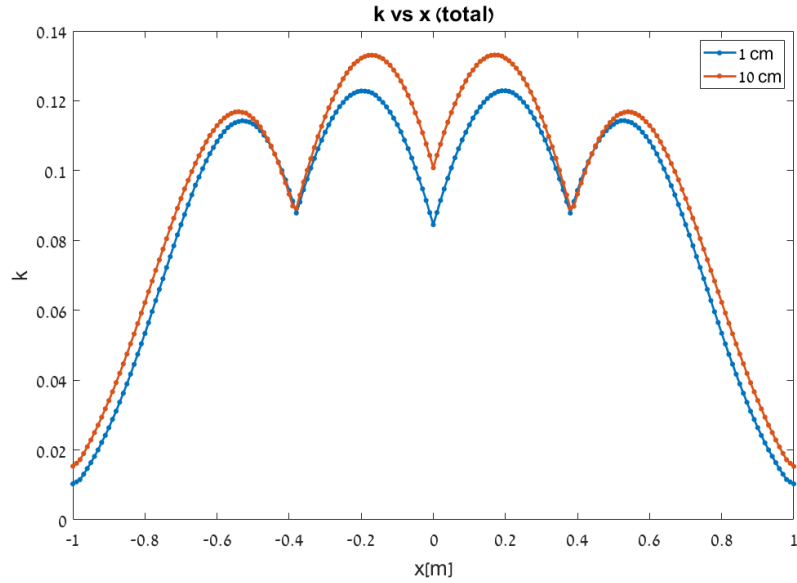
Figure 34: Changes to k at different x -axis misalignments for two spacing options – the default 1 cm case, and the 10 cm case, the latter being superior in every single way.
