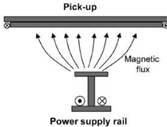
Figure 4: I-type transmitter configuration. The transmitter coil is wrapped around an I-shaped magnetic core, which helps to increase flux transfer by directing it upwards [25].
