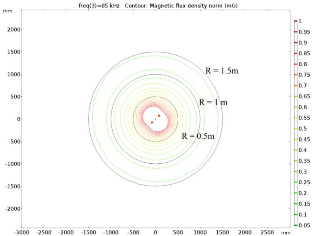
Figure 30 : Flux lines at 0.5m, 1m and 1.5m away from the cable. The lack of symmetry around the cable is a direct result of the opposite terminals of the cable, as seen in the previous figure.
