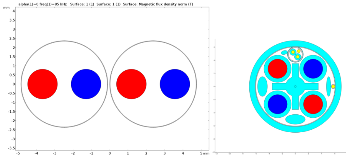
Figure 29: Simulated model of the cross-section of the cables. Left: Double twisted cable. Right: 4C cable. The red and blue colors represent positive and negative terminals respectively.
