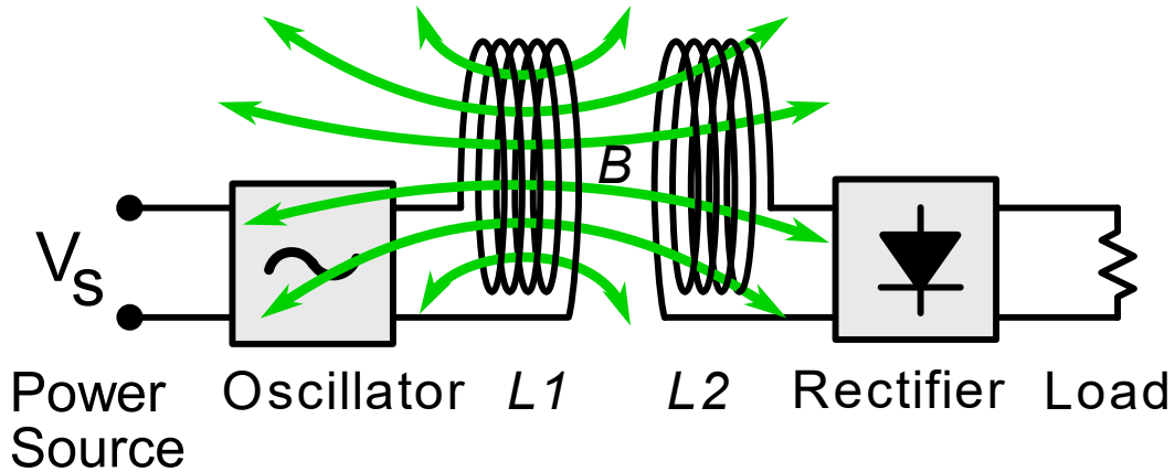
Figure 1: Inductive Power Transfer. The transmitter coil L_1 is connected to an oscillator. Some of the magnetic flux is then picked up by the receiver coil L_2 , which is connected to the load [9].
