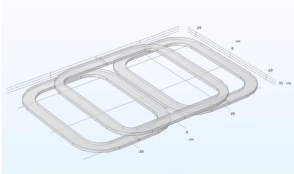
Figure 10: Simulated 'DDQ' Configuration of the receiver coils placed under the chassis of the EV.
