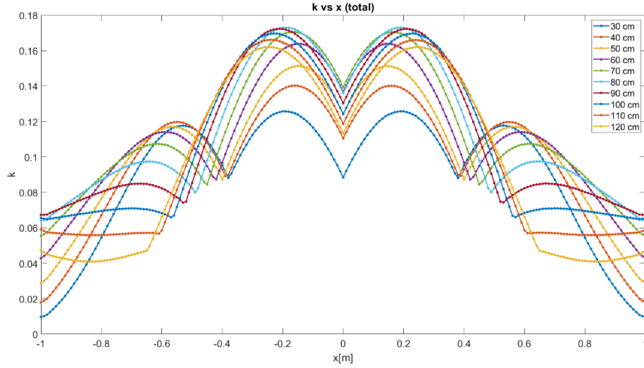
Figure 36: Changes to k dynamics with different sized coils.
