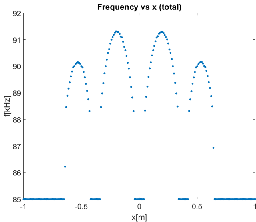
Figure 39 : Changes to the resonance frequency with misalignments in x for the initial configuration. Drastic changes to the resonance frequency are observed as k peaks.
