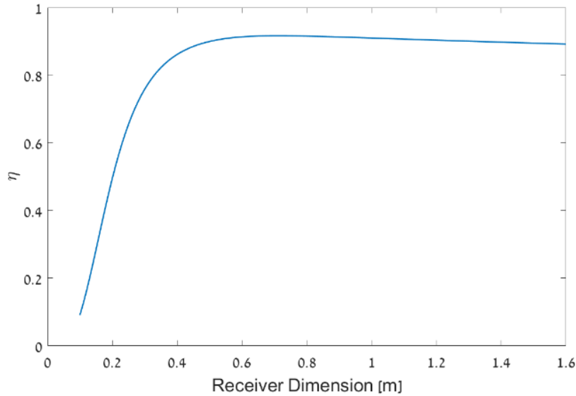
Figure 24: Energy transfer efficiency of the 10 cm separation case. It peaks at around 50-60cm, similarly to the peak in k shown in the previous figures. Unlike the previous figures however, the decline afterwards is rather small.
