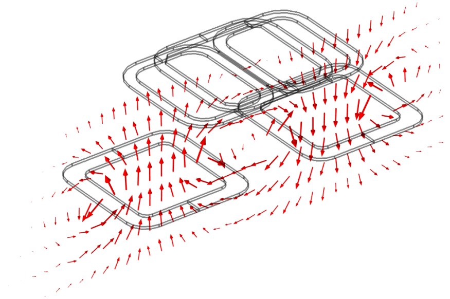
Figure 14: Flux lines generated in the bipolar transmitter coils. The lines are picked up by the 'DDQ' receivers.
