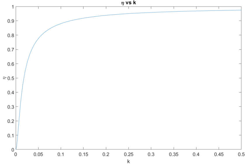
Figure 25: Efficiency changes with k . The efficiency is susceptible to changes for low k values.
