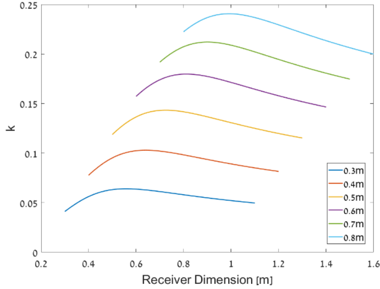
Figure 17: Coupling coefficient as a function receiver coil length. Different curves represent different transmitter coil dimension from 0.3 (lowest curve) to 0.8 m.
