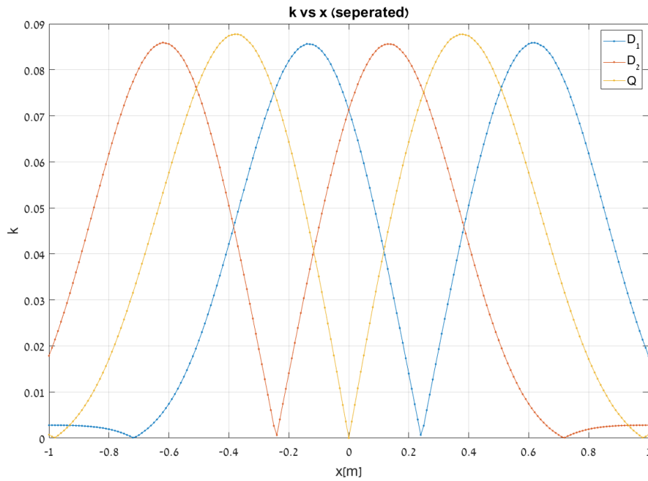
Figure 11: 'DDQ' configuration coupling coefficient as a function of travel path misalignment. Each coil effectively 'covers' for the 'dead zones' of the other coils, creating a sort of diode-bridge type of configuration.
