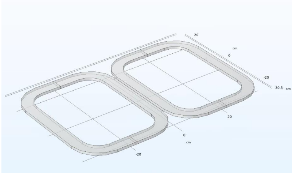
Figure 8: Simulated 'DD' configuration of the receiver coils placed under the chassis of the EV.
