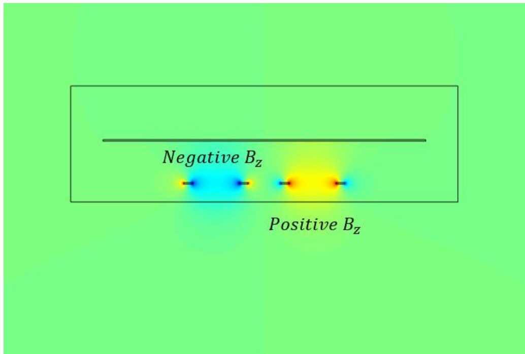
Figure 21: A side view of the system. Yellow hues represent positive z flux, while blue hues represent negative z flux.
