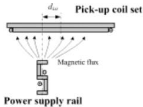
Figure 5: S-type transmitter configuration. The transmitter coil is wrapped around a S-shaped magnetic core instead, increasing the effective range of power transfer [26]. This configuration is superior due to the core's shape being more central, which in turn directs the flux lines more effectively into the receiver coils.
