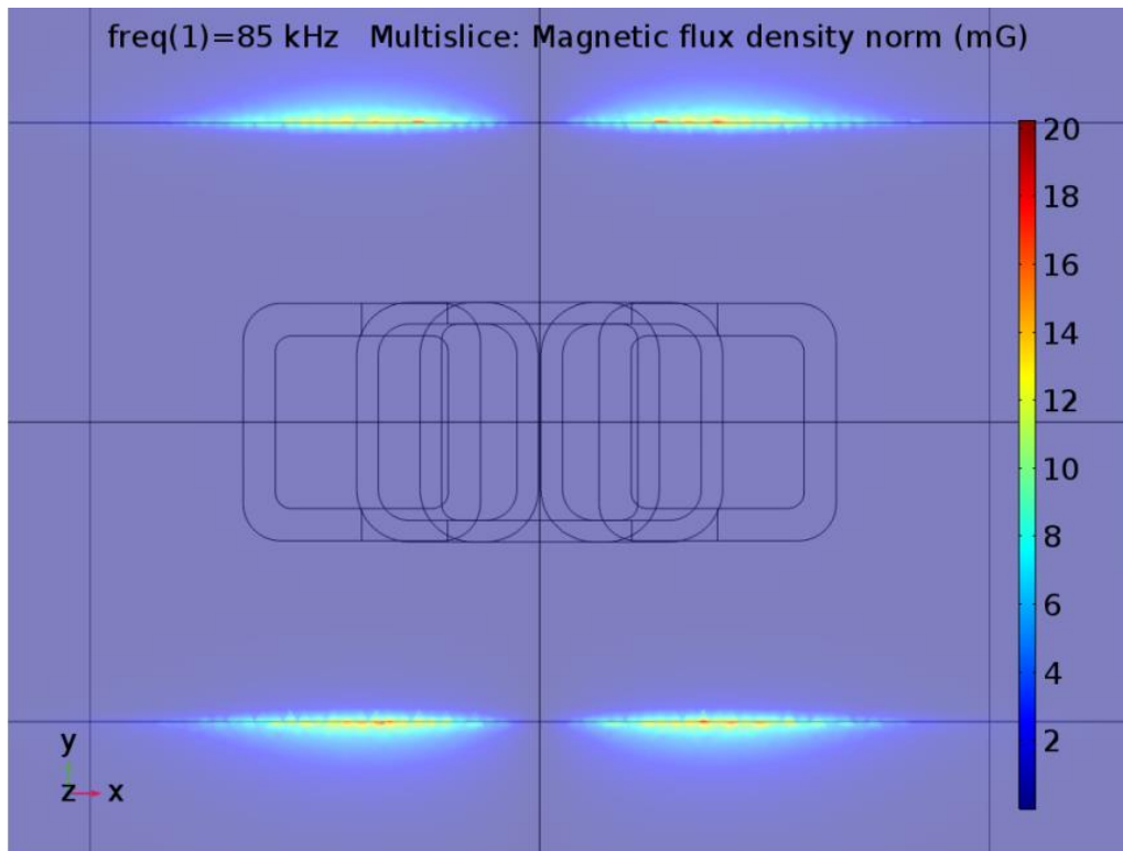
Figure 28: Radiation intensity (mG) at ferrite plate level. The maximal flux we get from the sides of the plate are well below the maximum allowed radiation levels. If needed, an aluminum plate can be placed to further reduce radiation.
