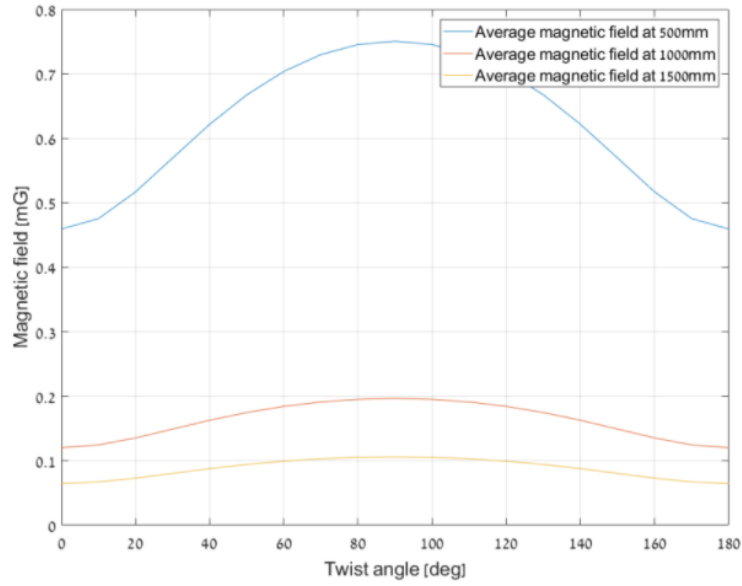
Figure 31 : Twist angle distribution of the flux in the double twisted cable. The x-axis represents the twist angle of the cable. The y-axis represents the residual average magnetic flux at different heights above the cable. At 0.5m the radiation is well below the allowed radiation levels.
