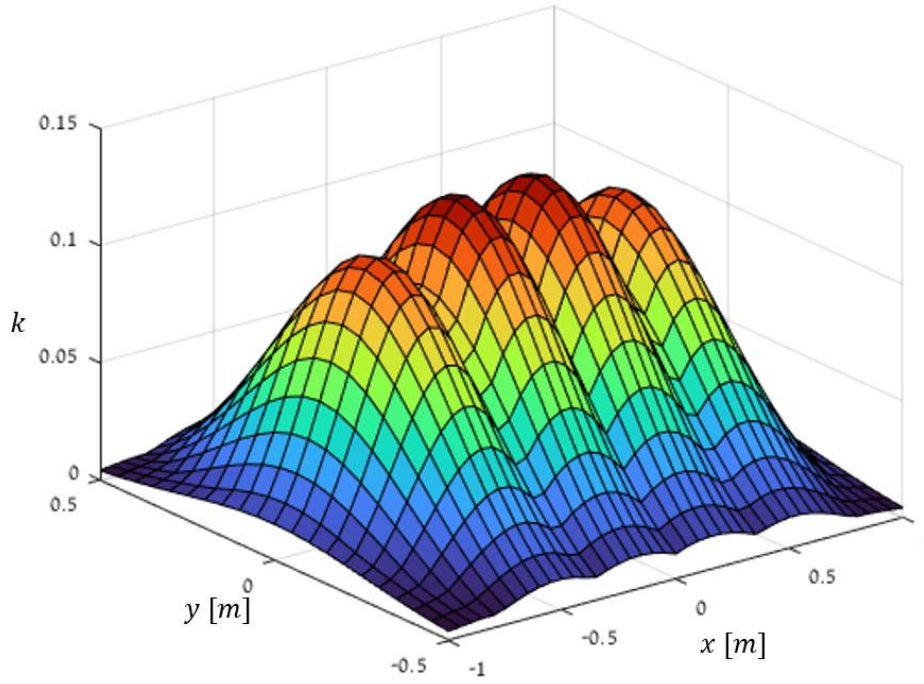
Figure 35: x-y mapping of k as a function of the misalignment in the x and y axes.
