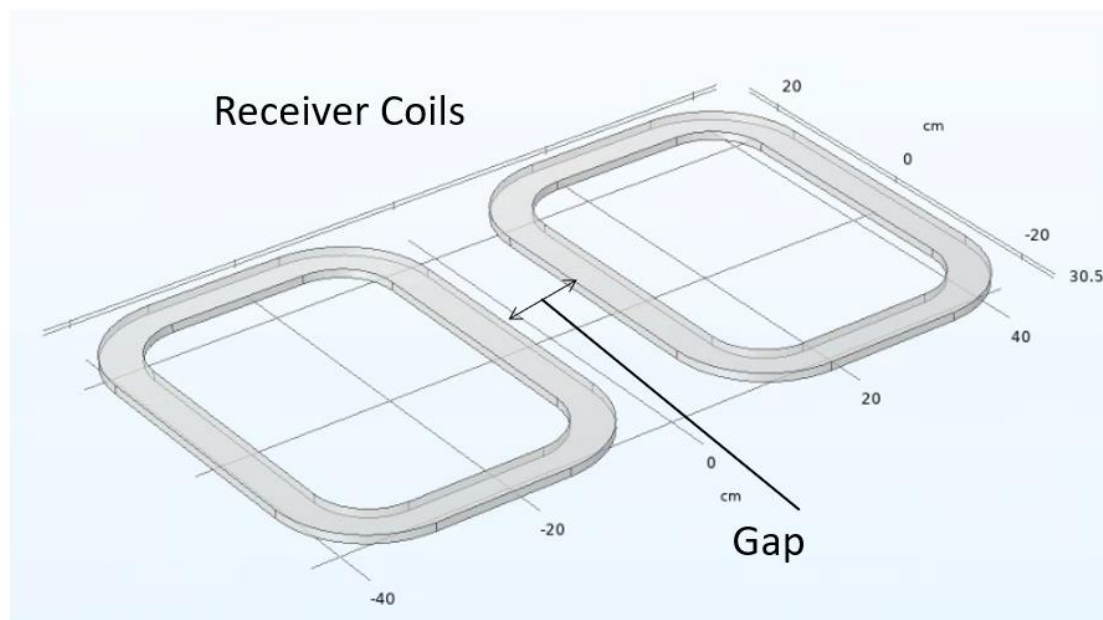
Figure 22: Added gap between the 'DD' coils.
