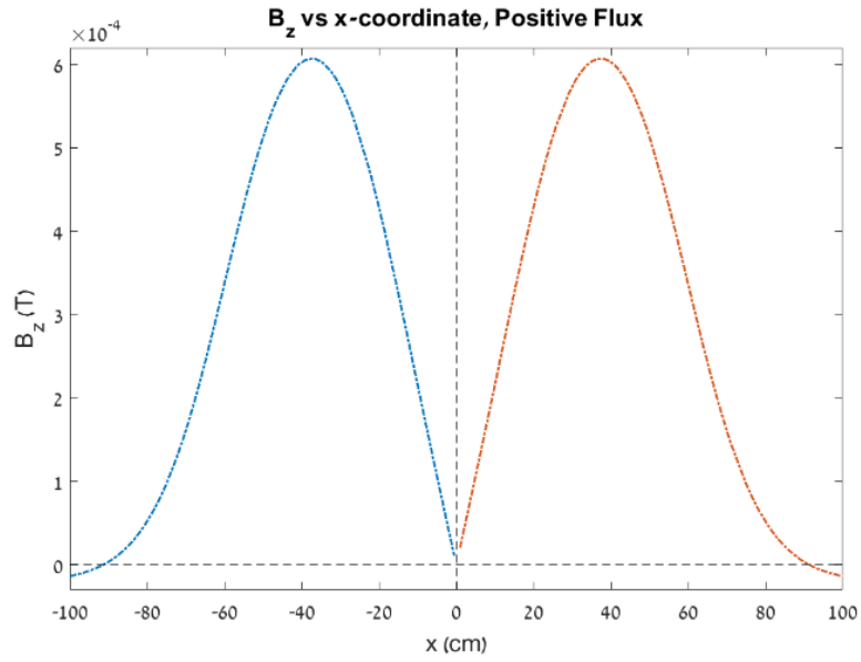
Figure 18: Position dependent B_z along the x-axis on the XY plane of the receiver. The direction of the flux displayed in this figure represents the flux that is seen by each receiver. Maxima are observed at around x = \pm 38 cm.
