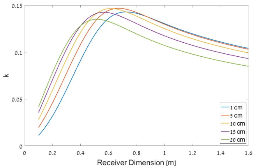
Figure 23: Comparison between different separating gaps.
