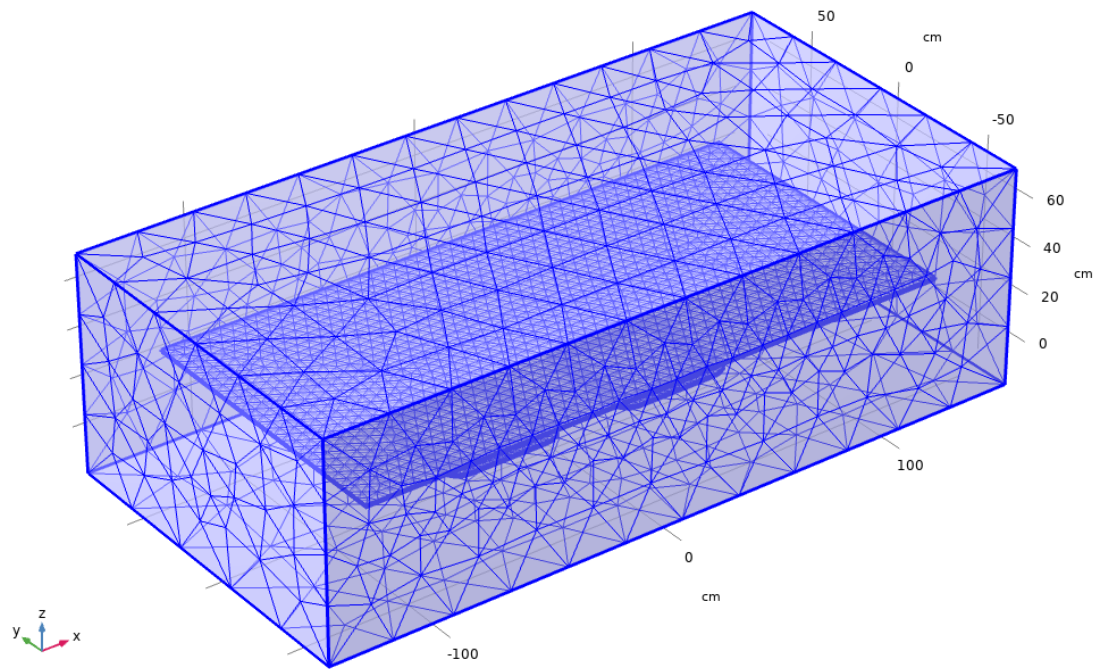
Figure 12: Mesh example for the simulated DWPT system. The outer block describes the ‘world’ in which the system lives in. It is simulated to be air. Inside this block, the receiver and transmitter coils are simulated, as well as the ferrite plate (flat rectangle inside the block). This link system is then converted into an adjacency matrix.
