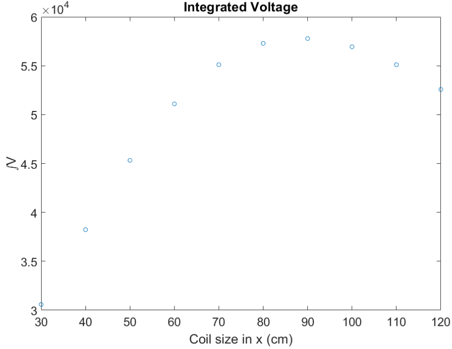
Figure 37 : Total integrated voltage for each size case. The maximum voltage was accumulated in the 90 cm case.
