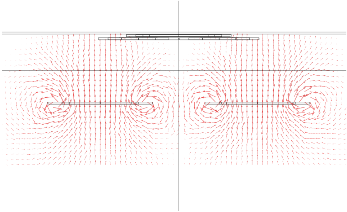
Figure 6: An example of the flux lines of a unipolar configuration, simulated by us. Each transmitter coil has a counterclockwise current applied to it. This results in spatial gaps in the flux field.
