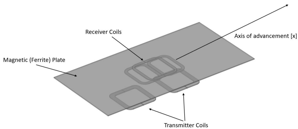
Figure 32 : Baseline configuration for the dynamic simulations. The axis of advancement is dubbed 'x' for the rest of this work.
