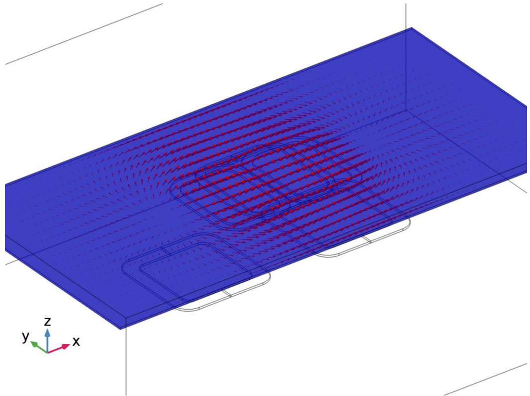
Figure 27: Flux lines inside the ferrite plate that screen the incoming radiation.
