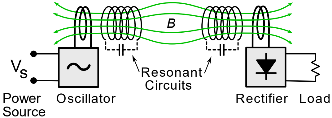
Figure 2: Resonant inductive power transfer. Both transmitter and receiver coils are connected to a resonator, meaning the power transferred between them is vastly increased [9,11].
