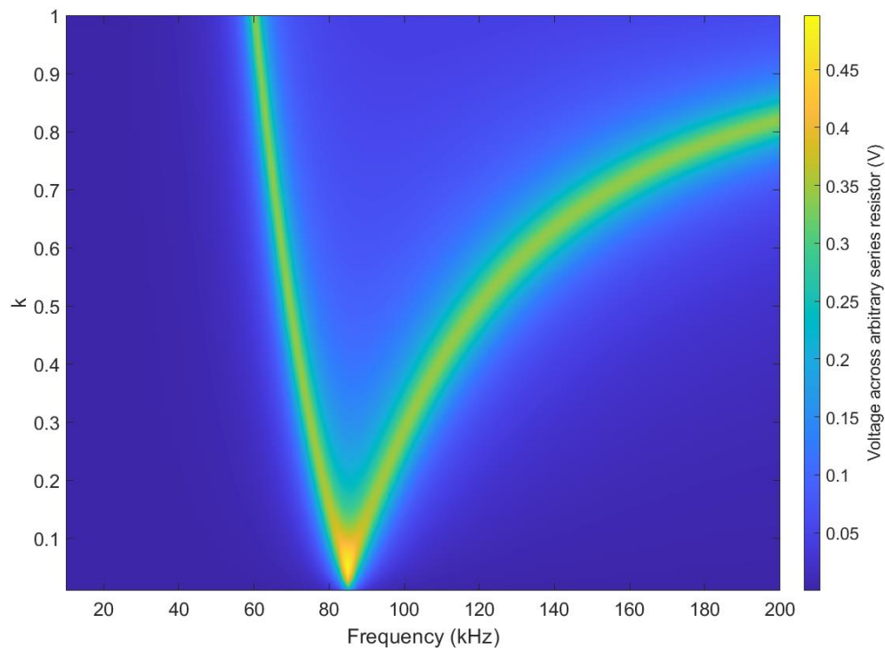
Figure 38: Resonance split occurs if the coupling becomes strong enough. The x-axis represents the resonance frequency of the system. The y-axis represents the coupling coefficient. The color-bar represents the effective voltage induced in the receiver coils. Instead of a single resonance frequency, two applicable resonance frequencies emerge. This must be considered when designing the electronics and circuitry of DWPT systems.
