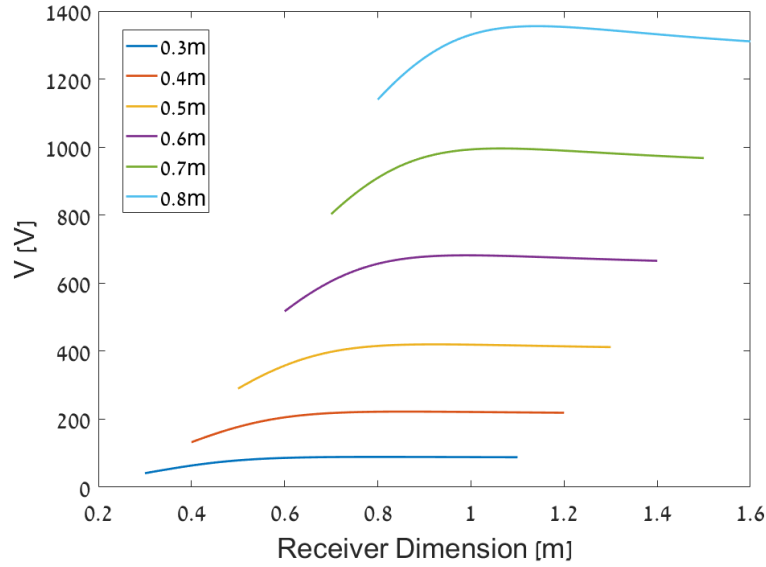
Figure 16: Length dependent receiver voltage. Different curves represent different transmitter coil dimensions from 0.3 to 0.8 m
