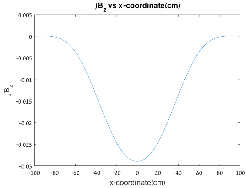
Figure 19: Integrated z component of the magnetic flux density along the x-axis.
