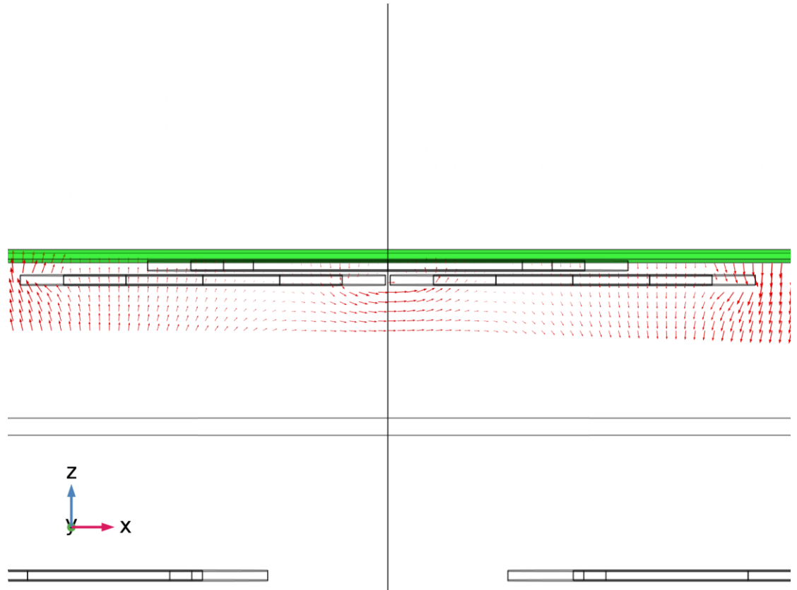
Figure 26: A side view of the system. Flux lines are drawn in proximity to the ferrite plate in a logarithmic scale, including the region above it. This means that the flux above the ferrite is orders of magnitude lower than the incoming flux.
