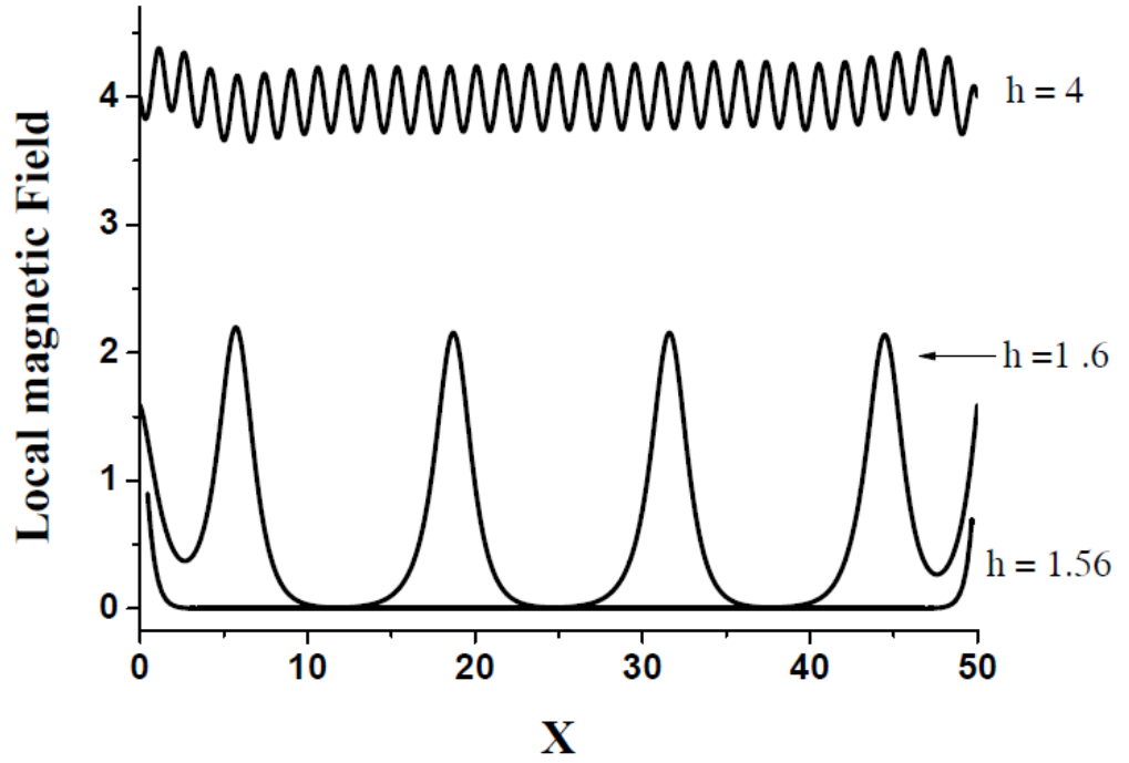
Fig. 2 Magnetic induction across a Josephson channel for \eta = 0.5 , and \alpha = 0.27 . Lowest curve: h = 1.56 , just below the Josephson critical field; Middle and upper curves, respectively: h = 1.6 and h = 4 , demonstrating soliton-like and large wave amplitude distribution.
