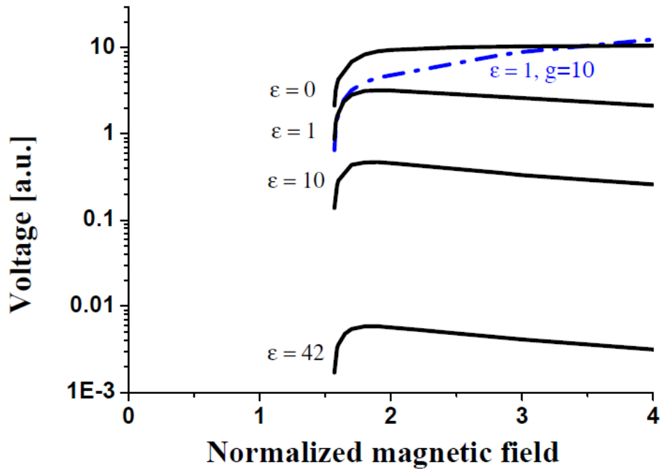
Fig.3. Solid curves: Calculated voltage in arbitrary units versus external magnetic field normalized to H_J for different values of the parameter \varepsilon taking the normalized current \alpha = 0.27 and a = 0.5 . The solid lines correspond to g = 0 . The dashed-blue curve is calculated for \varepsilon = 1, g = 10 .
