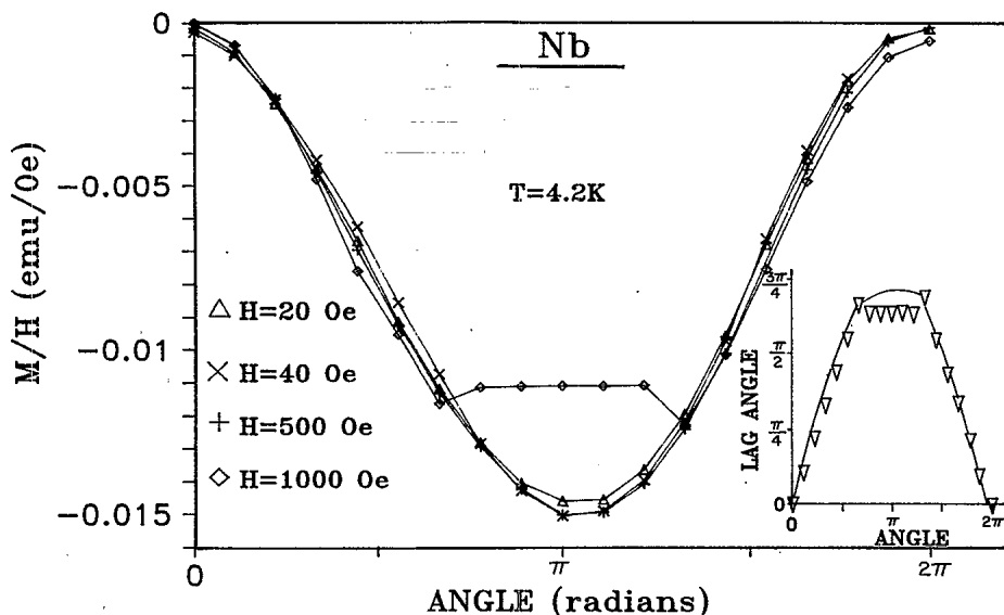
FIG. 5. Angular dependence of the field-cooled magnetization at 4.2 K for various fields for a Nb sample. Inset shows the lag \phi-\theta as a function of the rotation angle \phi for H=1\text{ kOe} .
