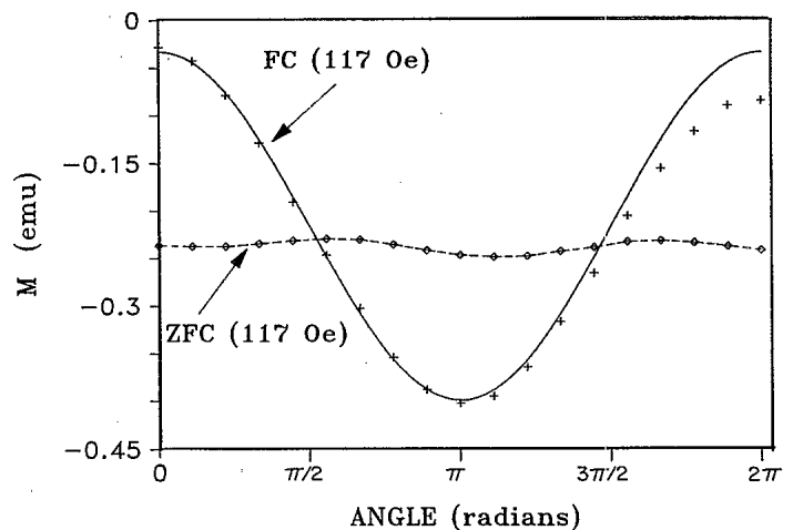
FIG. 1. Angular dependence of the field-cooled (FC) and zero-field-cooled (ZFC) magnetization in \text{YBa}_2\text{Cu}_3\text{O}_7 at 4.2 K for H=117 Oe. The solid line among the FC data points is a result of a least-squares fit according to Eq. (2) (see text).
