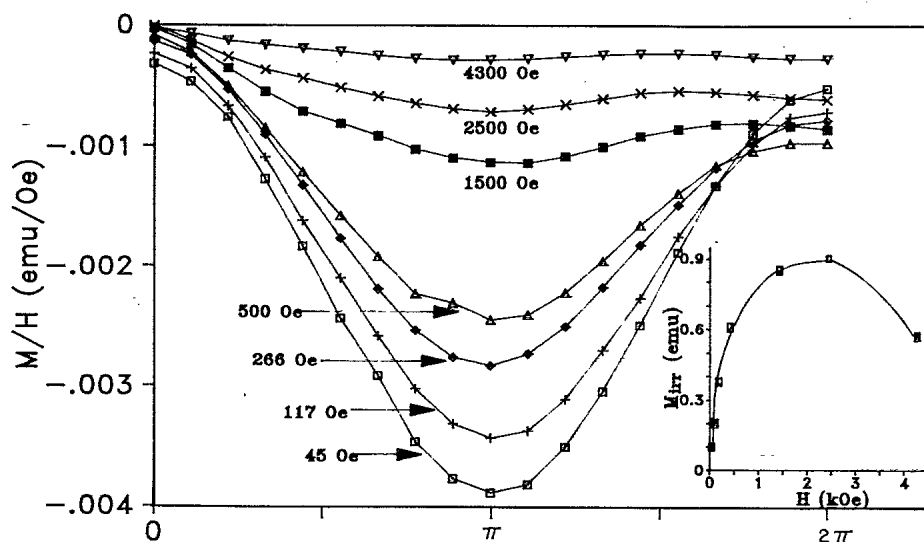
FIG. 2. Angular dependence of the field-cooled magnetization for \text{YBa}_2\text{Cu}_3\text{O}_7 at 4.2 K for various fields. The solid lines are a guide for the eye. Inset shows the field dependence of M_{\text{irr}} deduced from the angular dependence data (see text).
