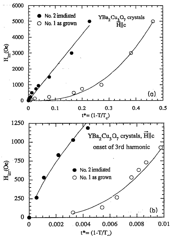
FIG. 3. The irreversibility lines (IRL) of \text{YBa}_2\text{Cu}_3\text{O}_7 samples before (open symbols) and after (solid symbols) irradiation. (a) The IRL determined by dc technique, from ZFC and FC magnetization curves. (b) The IRL determined from the onset of third harmonics in the ac response. The solid lines are theoretical fits, assuming a power-law dependence of the field on the reduced temperature.
