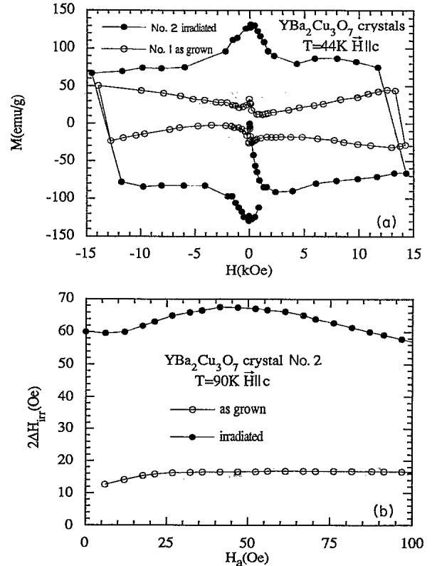
FIG. 1. Magnetization curves and width of hysteresis loop of YBa _2 Cu _3 O _7 samples before (open symbols) and after (solid symbols) irradiation. (a) Magnetization curves at 44 K, recorded with the VSM for samples 1 and 2. (b) Width of magnetization curves at 90 K for sample 2, measured by the local Hall-probe technique.
