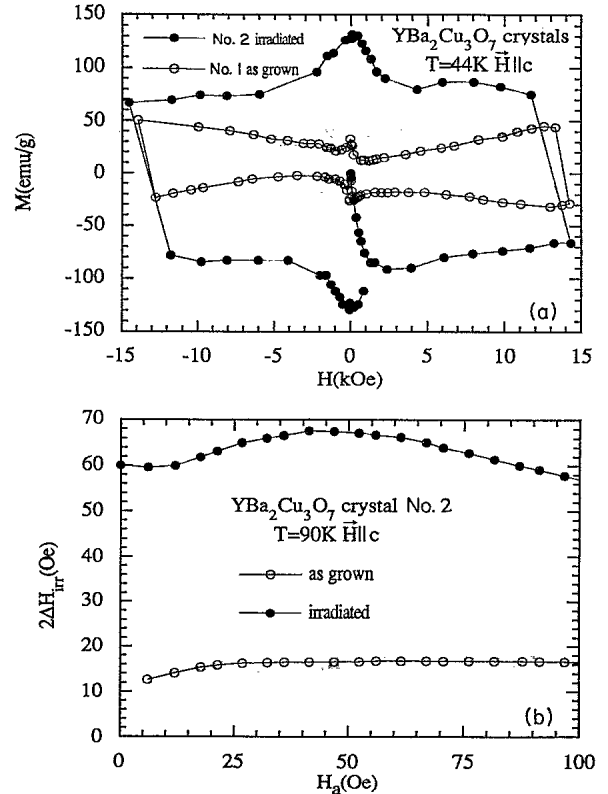
FIG. 1. Magnetization curves and width of hysteresis loop of YBa 2 Cu 3 O 7 samples before (open symbols) and after (solid symbols) irradiation. (a) Magnetization curves at 44 K, recorded with the VSM for samples 1 and 2. (b) Width of magnetization curves at 90 K for sample 2, measured by the local Hall-probe technique.
